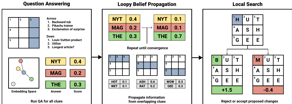
Figure 2: An overview of the Berkeley Crossword Solver. We use a neural question answering model to generate answer probabilities for each question, and then refine the probabilities with loopy belief propagation. Finally, we fill the grid with greedy search and iteratively improve uncertain areas of the puzzle using local search.
