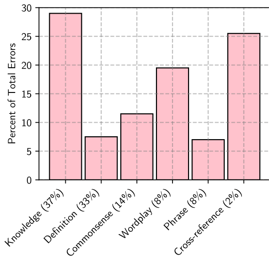
Figure 6: We manually categorize our QA failures using the categories from Table 1. The rate at which each category occurs in random examples is shown in parentheses. A disproportionate fraction of QA errors are due to cross-reference and wordplay clues.
