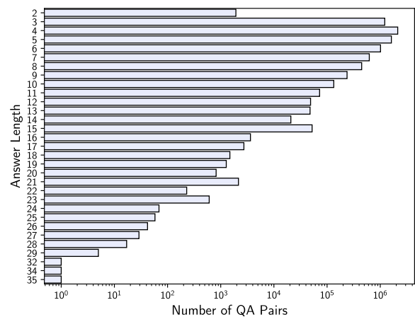
Figure 9: The answers in our dataset span many different lengths; longer answers are typically more difficult multi-word expressions or theme answers.
