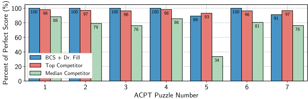
Figure 5: A breakdown of our 2021 ACPT performance. The 2021 ACPT consisted of 7 puzzles, for which our combined system achieves a perfect score and surpasses the top human competitor on 5 out of the 7 puzzles. We include the median competitor’s performance to illustrate the difficulty of the puzzles.
