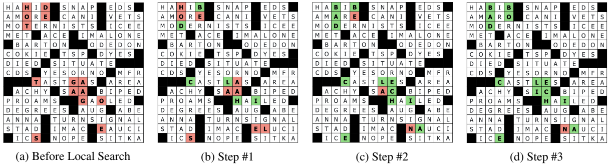
Figure 4: We show the result of our solver on a NYT puzzle after running greedy search and three consecutive steps of local search. Local search considerably improves accuracy but fails to fix the answer regarding Dr. Fauci (an error due to temporal shift in our QA models). Red squares indicate errors from the output of greedy search, while green squares indicate corrections from the local search. See Figure 12 for the clues and associated answers in the puzzle.
