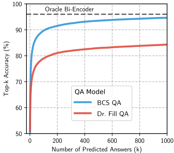
Figure 3: Top-k accuracy on the 2021 NYT test set. Dr.Fill QA is an existing crossword QA system that ensembles TFIDF-like scoring with numerous additional scoring modules. Our neural bi-encoder model improves top-1000 accuracy from 84.4% to 94.6%.
