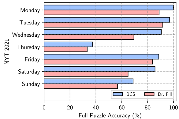
Figure 10: We compare our system’s accuracy on NYT puzzles to the previous state-of-the-art Dr.Fill system and break down the results by day of the week. Both systems succeed on early week puzzles but struggle on Thursday puzzles that often contain unusual themes.
