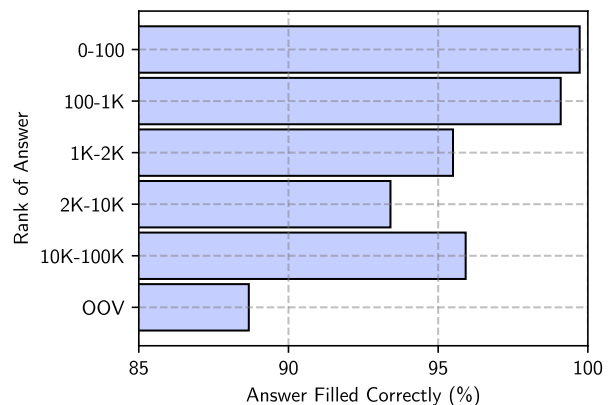
Figure 11: The chance that the BCS correctly fills in an answer as a function of the rank of the answer under its QA model. If the QA model predicts the answer in its top 1,000 candidates, it is usually filled in correctly.
